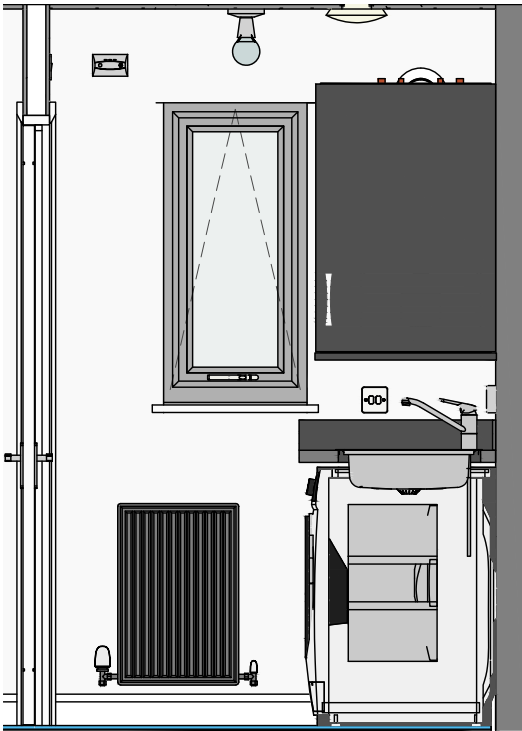
A Kitchen - View B 1 : 25
